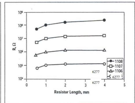
Figure 8. Length Effects
